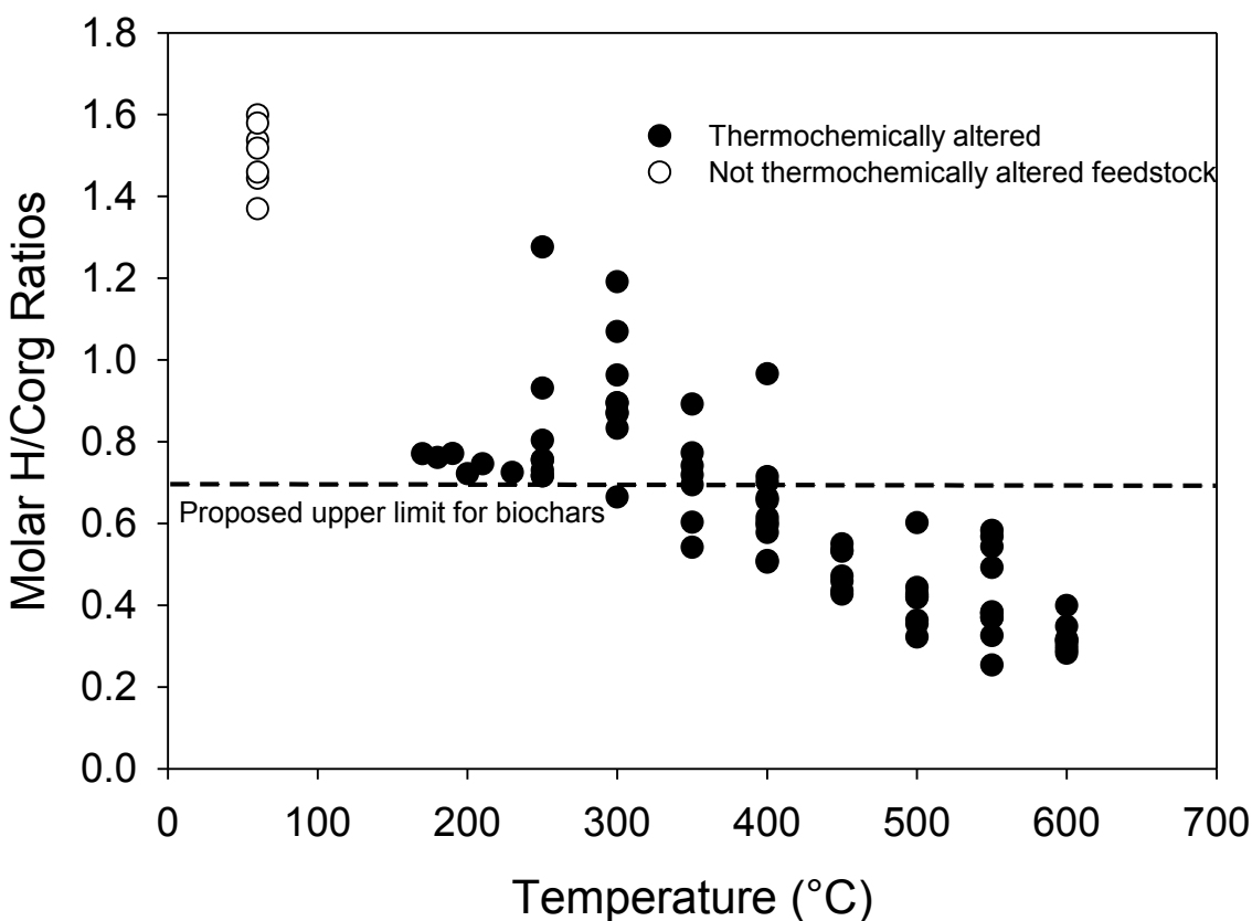
Figure A5.1: Relationship between molar H:C org ratios and temperature of thermochemically altered organic matter in comparison to untreated biomass. Dashed line is the upper limit of 0.7. Data points below the 0.7 line are thermochemically altered materials that are considered to be thermochemically “converted” (data from Sevilla and Fuertes, 2009ab; Calvelo Pereira et al, 2011; Enders et al., 2012).
